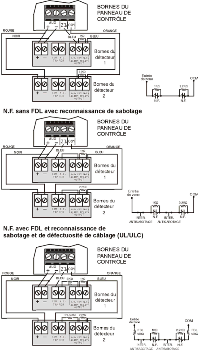
Figure 2-7 : Raccordement de zones doublées
